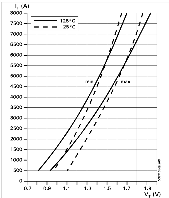
Fig. 2. On-state characteristics.
