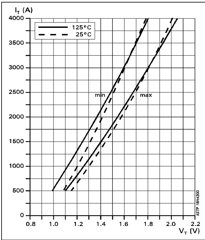
Fig. 2 On-state characteristics.
