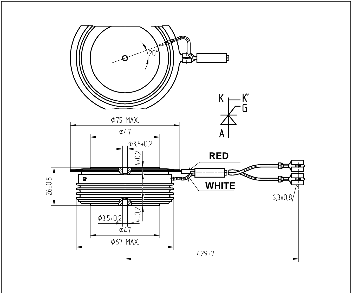
Fig. 10 Device Outline Drawing.
