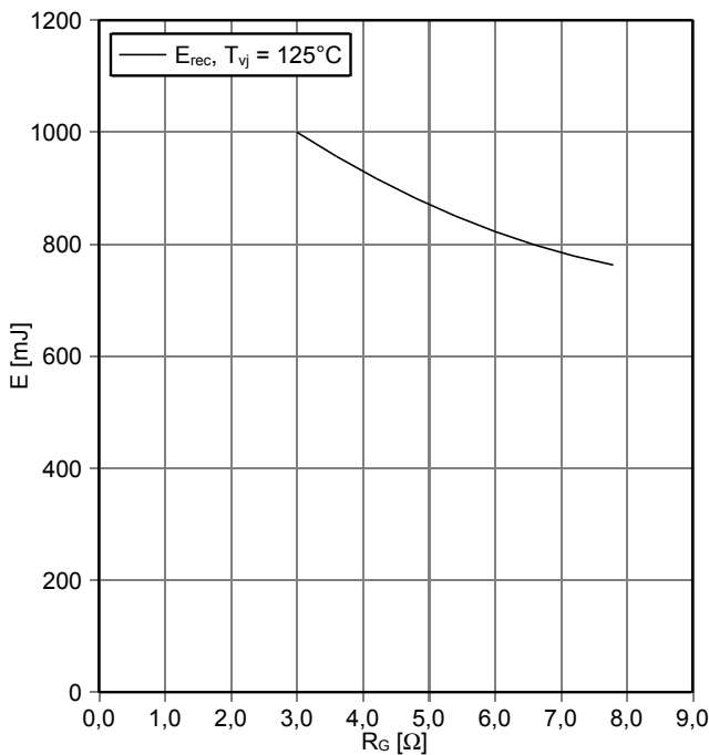
Schaltverluste Diode, Brems-Chopper (typisch) switching losses Diode, Brake-Chopper (typical) E_{rec} = f(R_G) I_F = 250 A, V_{CE} = 3600 V
