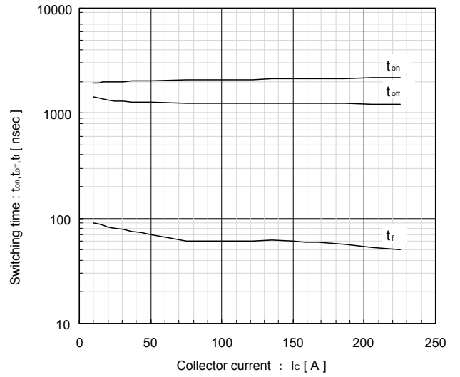
Switching time vs. Collector current (typ.) V_{bc}=300V, V_{cc}=15V, T_j=125^\circ C
