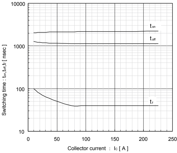
Switching time vs. Collector current (typ.) V_{bc}=300V, V_{cc}=15V, T_j=25^\circ C
